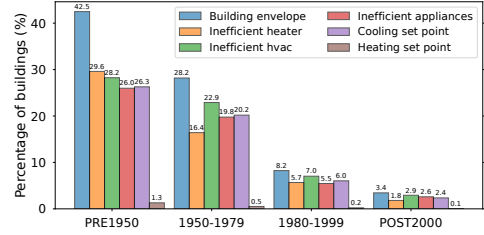
Fig. 8. Distribution of energy inefficiencies across buildings by age group.
