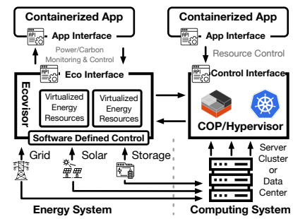
Fig. 2: Ecovisor’s architecture.
